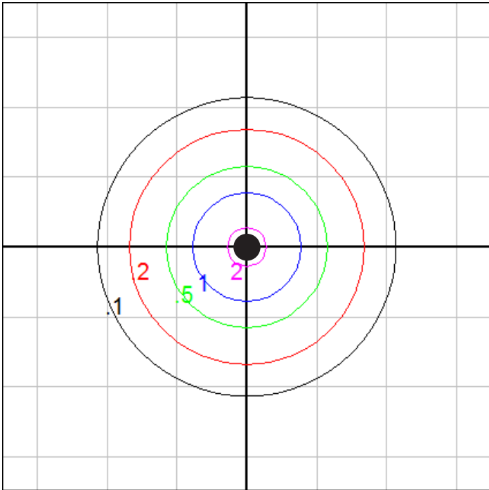
Ceiling Mount Fixture - Isofootcandle grid on floor Mounting Height = 10 ft. Grid Spacing = 10 ft.
