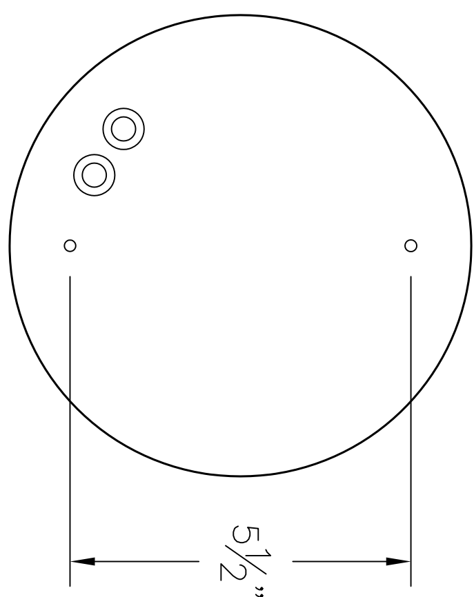
MOUNTING DETAIL
