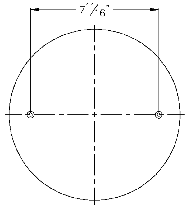
MOUNTING DETAIL
