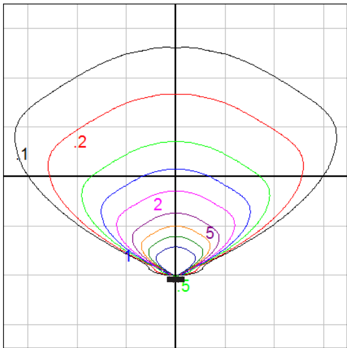
Wall Mounted Fixture - Iso-Grid on Wall Grid Spacing = 2.5 ft.
