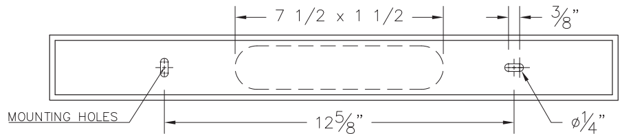
MOUNTING DETAIL
