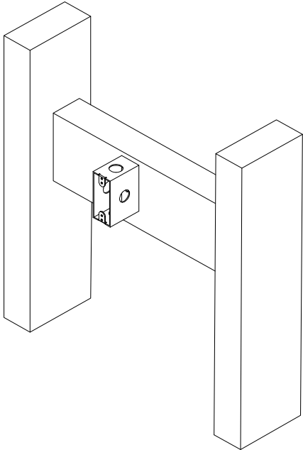
Figure 1: Mounting Detail
